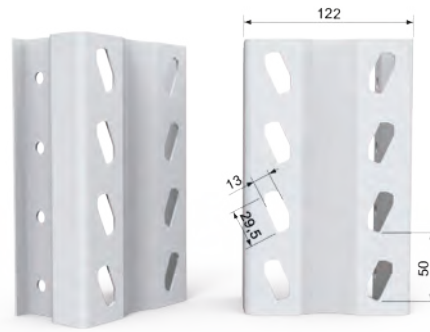
HX 122 PILLAR PROFILE
