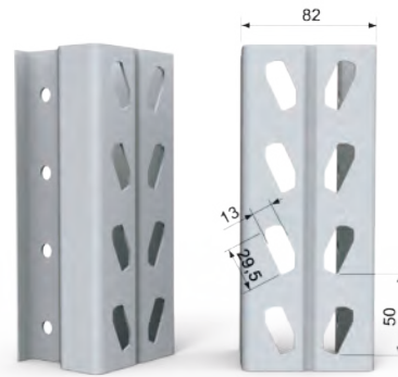
HX 82 PILLAR PROFILE
